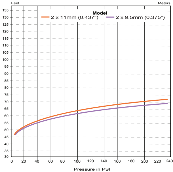
Effective Jet Throw Length
