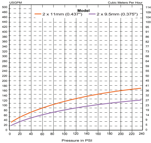
Flow / Pressure
