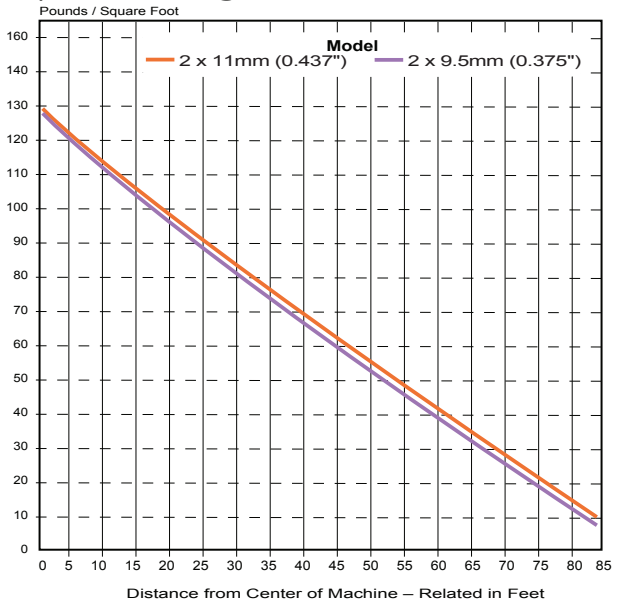
Impact Pressure @ 100 PSIG
